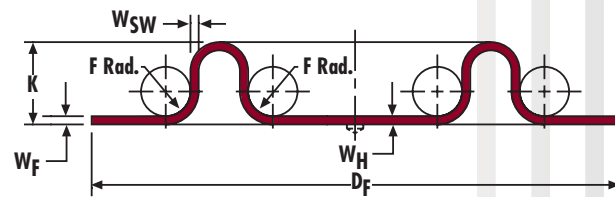
Fig. 10: Preconvoluted Diaphragm
