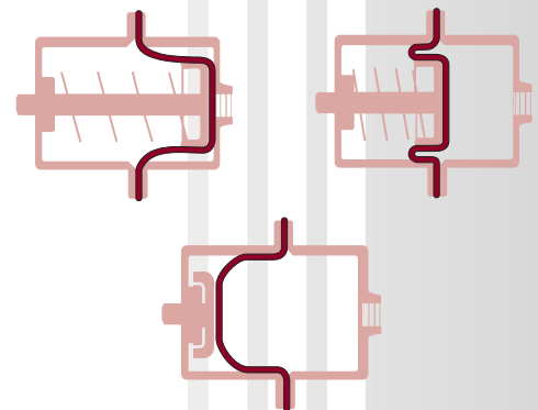
Fig. 13: Involved Diaphragm cycle. Convolution is not required at stroke limits.
